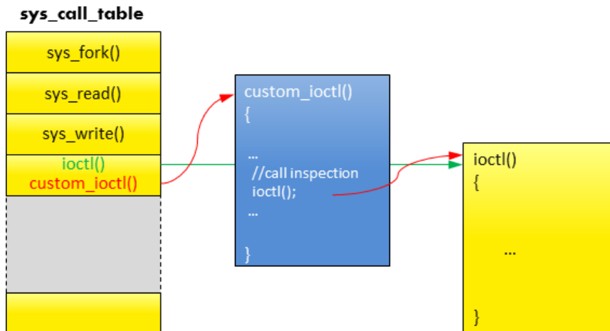
Figure 2: ioctl interception
