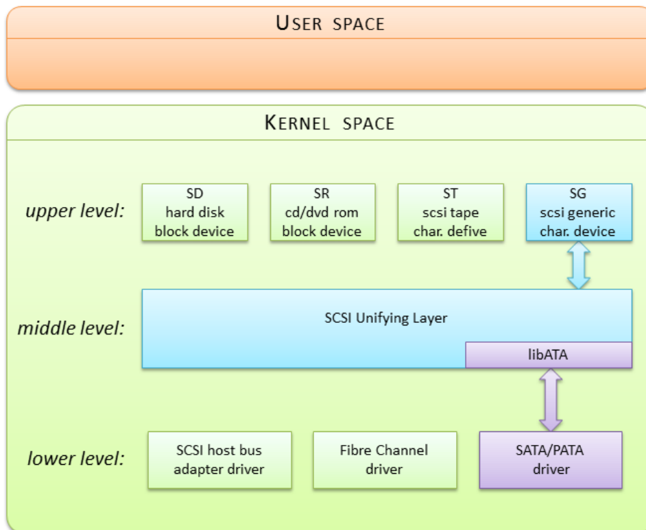
Figure 1: Linux storage driver layers
