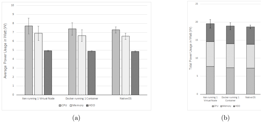
Figure 5: (a): Average Power Usage in Watt (W) when IDLE
