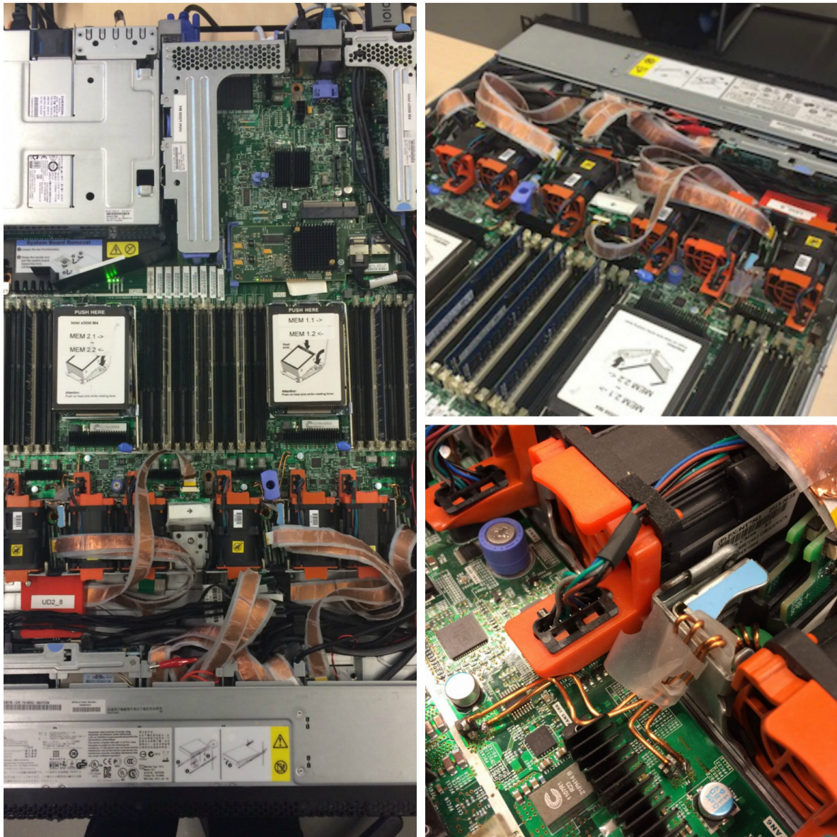
Figure 14: Physical Server
