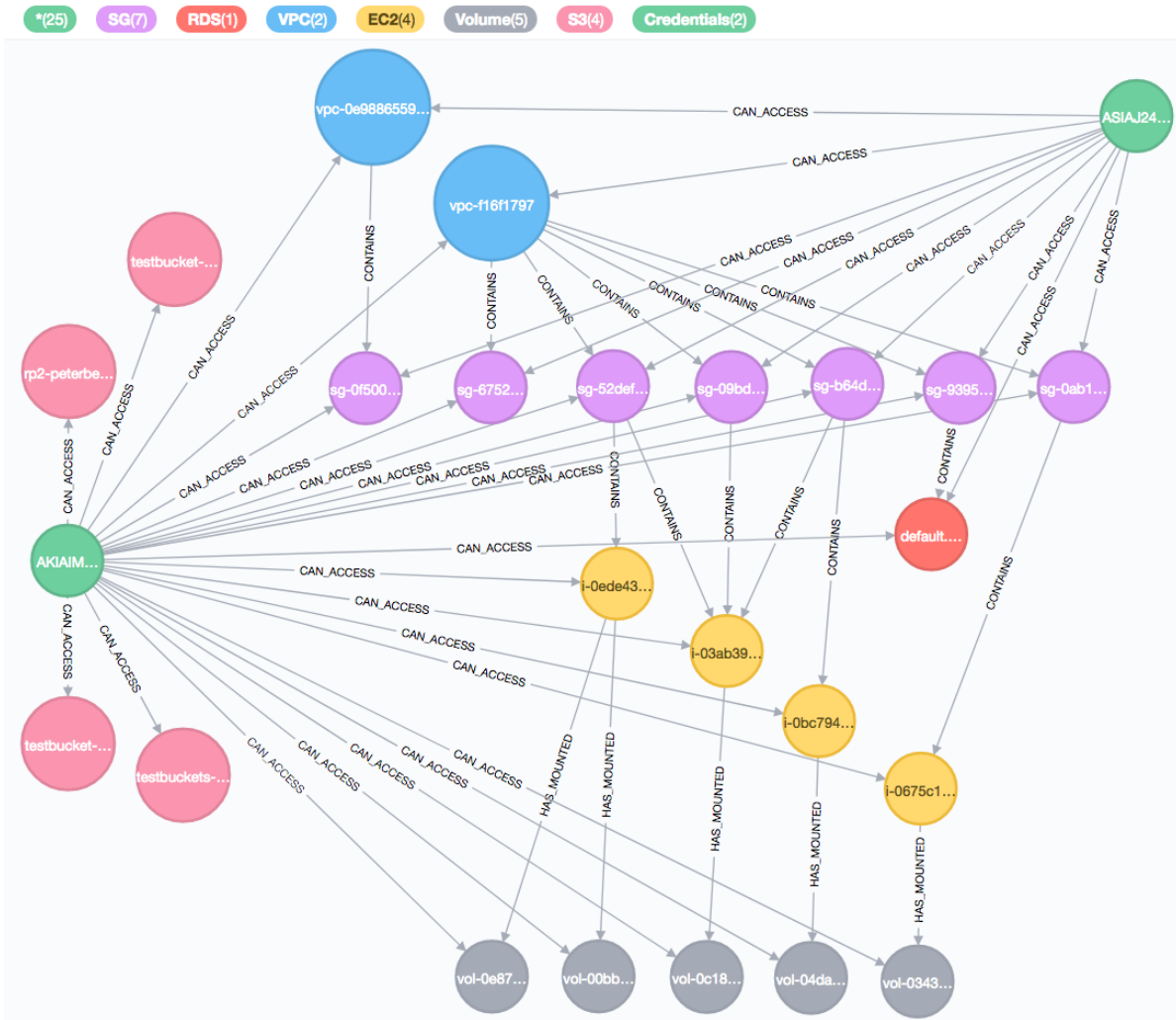
Figure 2: Output of Neo4j query for example infrastructure.
